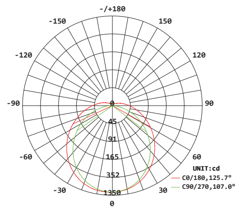
AVERAGE BEAM ANGLE(50%)-116.4 DEG TDL-DGA00-530WT-G8-T Plus
